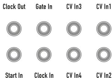
CV/Gate and Clock connections on the Iridium rear panel
