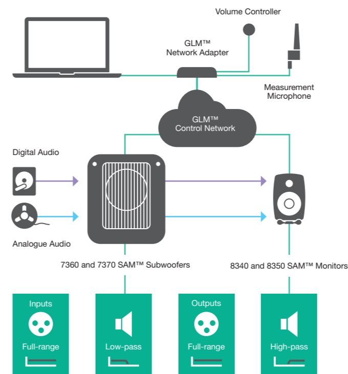
SAM™ System's basic connections and functionalities
